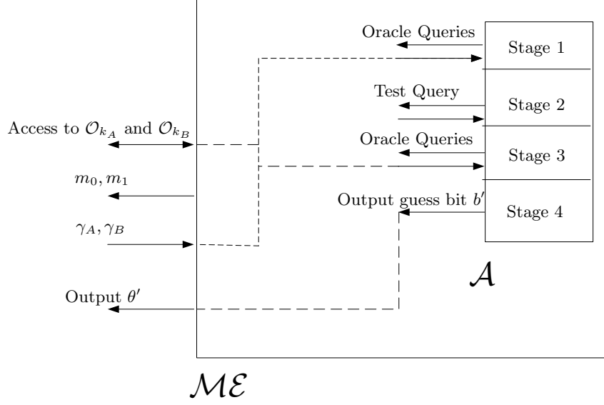
Fig. 5. Game \mathcal{G}_{\mathcal{M}\mathcal{E}}
